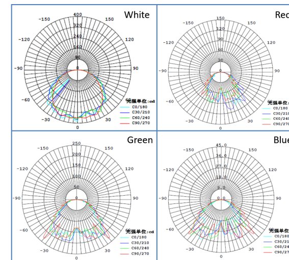
ISOLUX DIAGRAM
